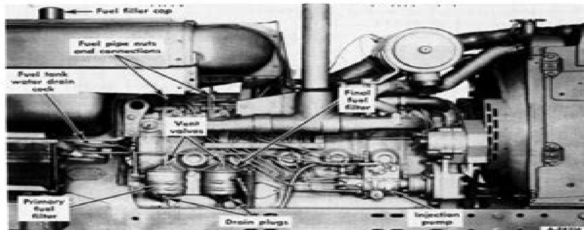
Illustr. 17 Fuel system on the right side of the diesel engine.
