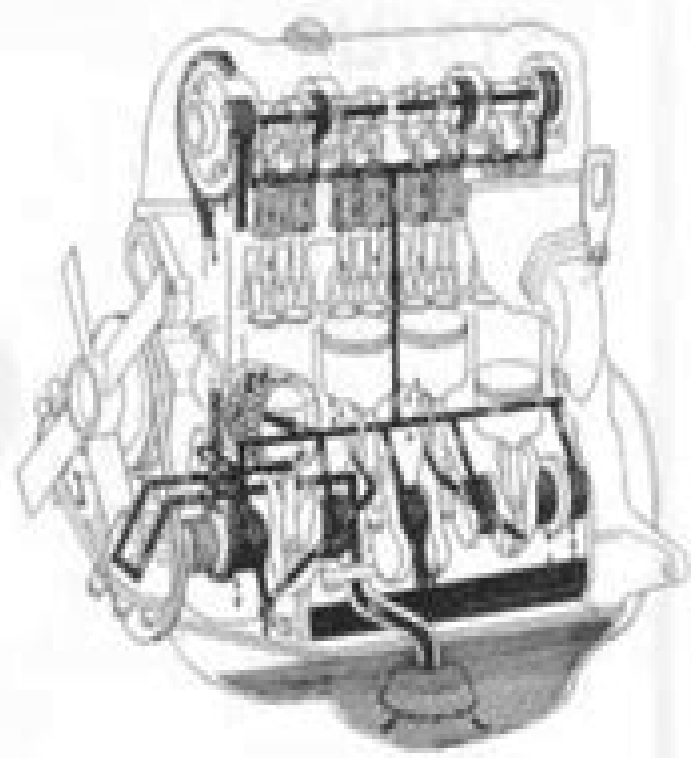
EL-001 Fig. EL-1 Lubricating circuit
